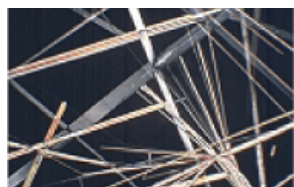
Vitamin E in its crystalline form
