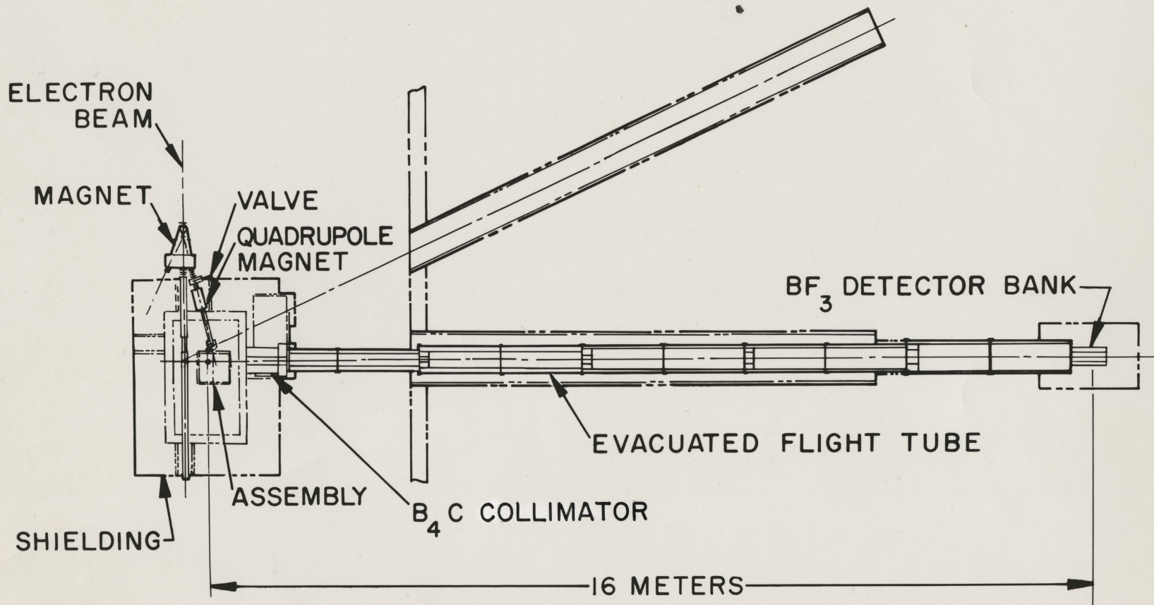
GEOMETRY FOR PULSED SPECTRUM MEASUREMENT
