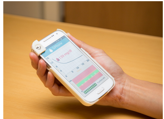
Custom-designed Android app displays test results on a smartphone screen
