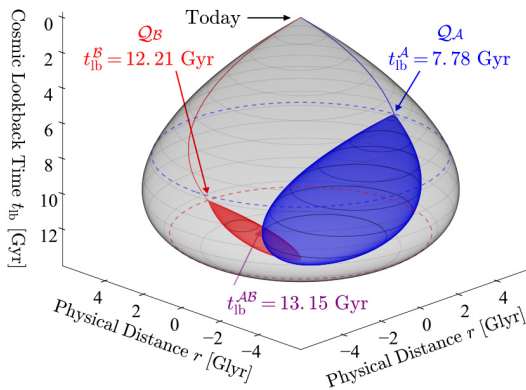
Diagram of a run of the Cosmic Bell test. The regions of space and time where an alternative, non-quantum mechanism could still have acted (limited to the red and/or blue regions) corresponds to at least 7.78 billion years ago (blue region). Light from the more distant quasar was emitted 12.21 billion years ago (red region). Compared to the gray region, representing all of space and time prior to the experiment, the alternatives are limited to within four percent of the space-time volume since the Big Bang. Image by Andrew Friedman and David Leon
