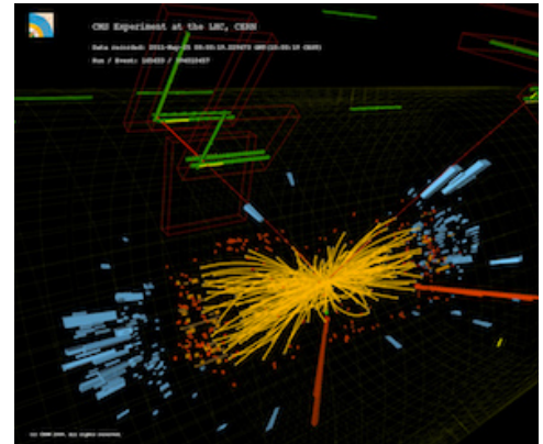
A Z boson, possible offspring of a Higgs, further decays in electrons (green streaks) and two muons (red lines). So far scientists aren't convinced that the events they've seen are blips in background noise. If enough accumulate they'll be they've found the Higgs. Image: CERN.
