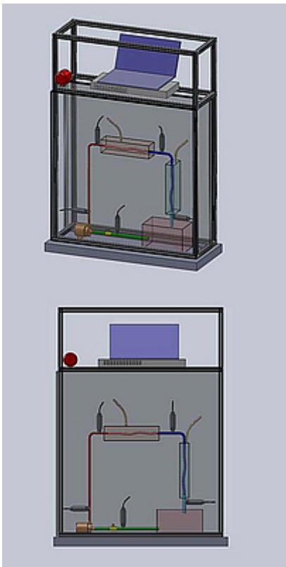
A computer-assisted drawing of the intracranial pressure modeling device.
