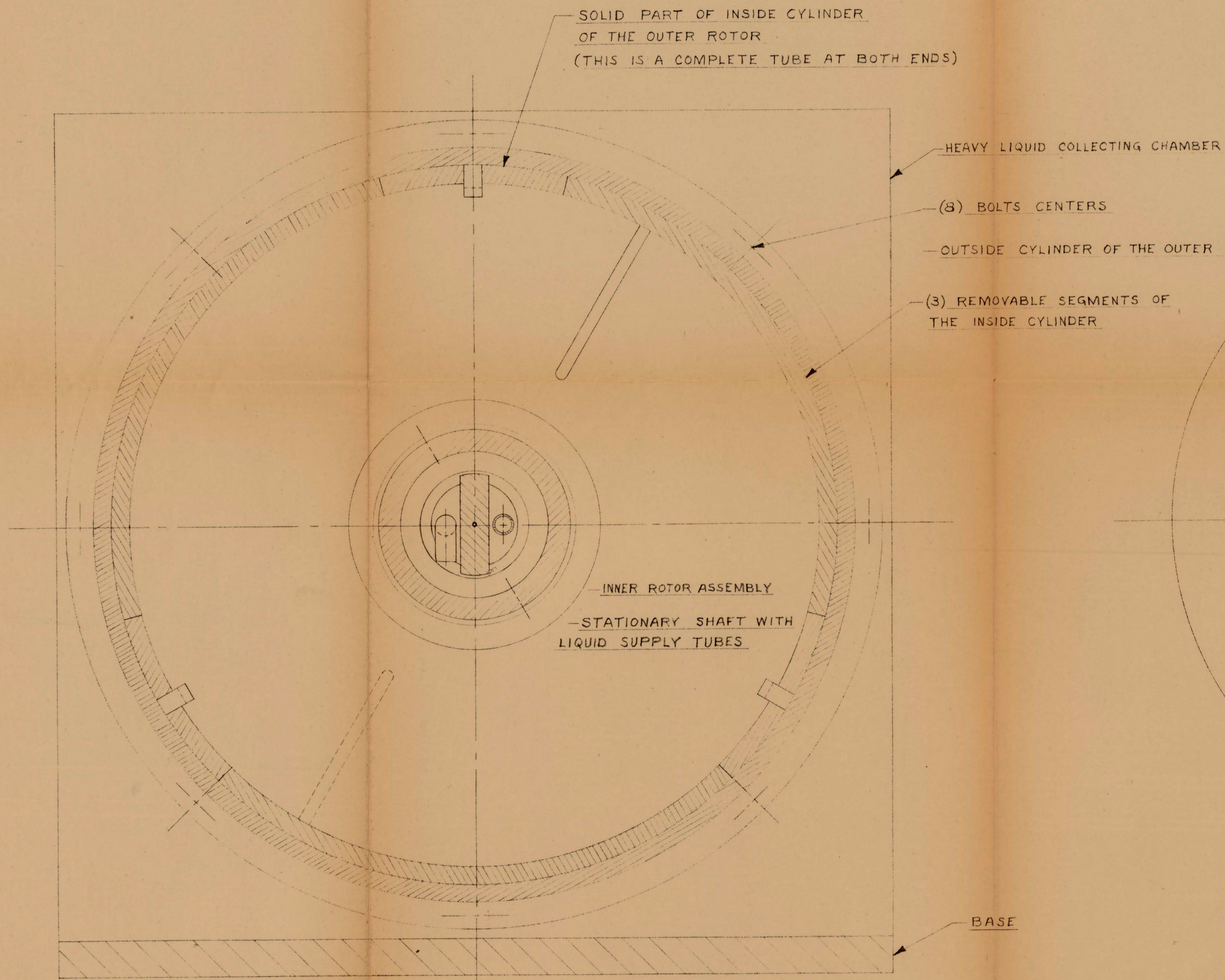
SECTION AA
