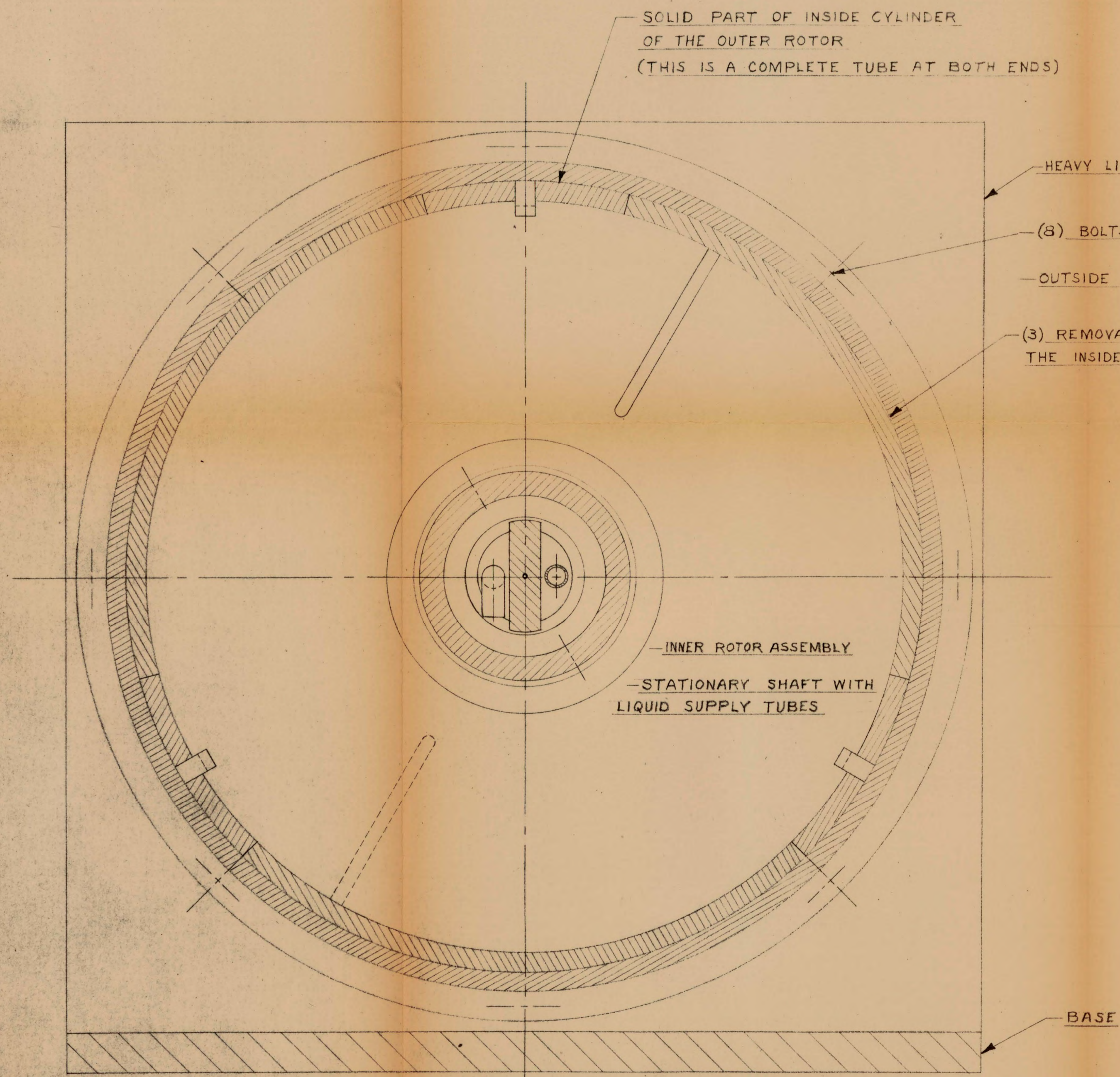
SECTION AA
