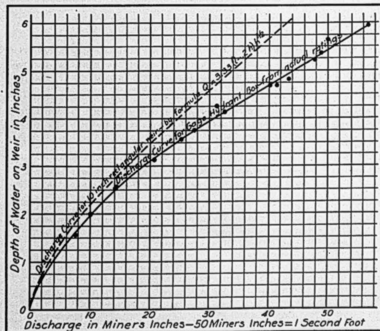
Rating Curve for Gage Hydrant
