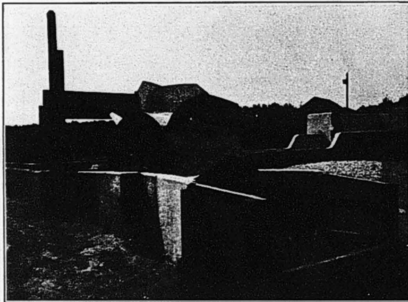
Fig. 20.—Photograph of Dethridge meter
