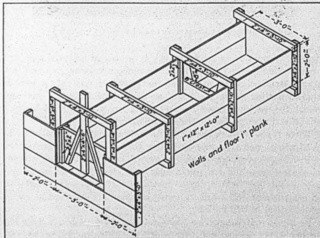
Fig. 12.—Drawing of Cipolletti weir and weir box
