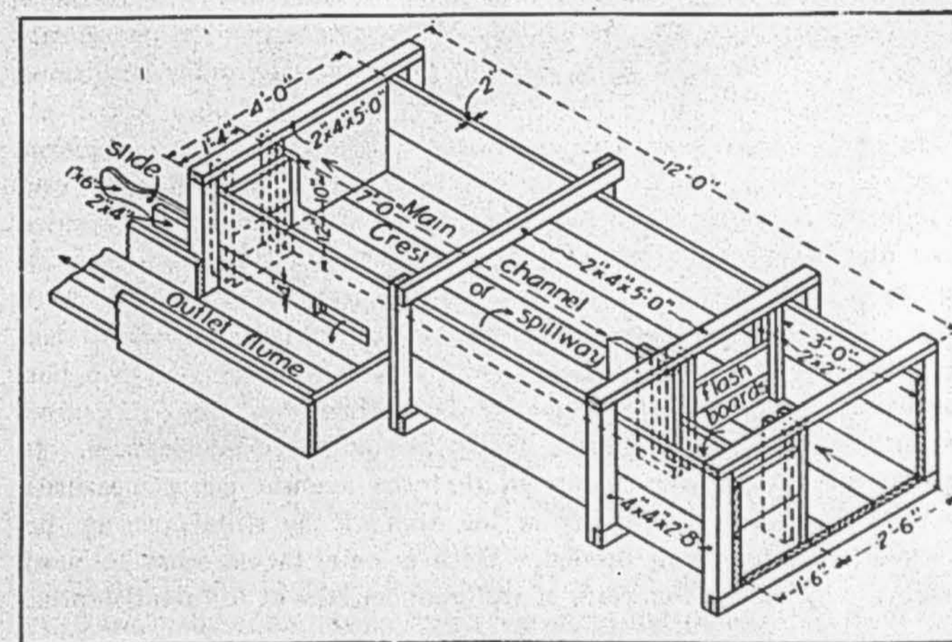
Fig. 9.—Drawing of Foote inch box
