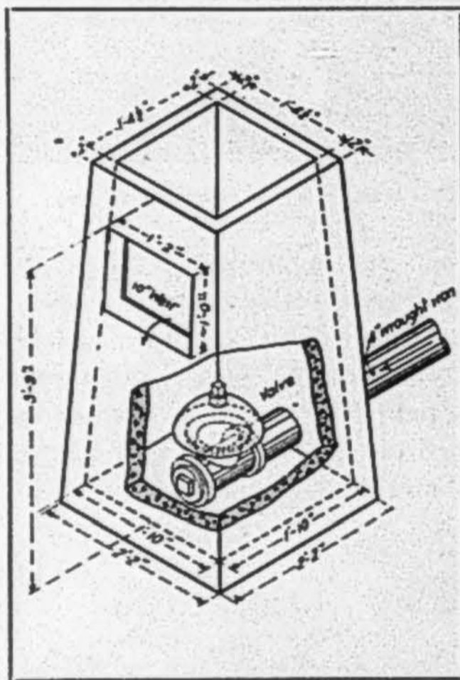
Fig. 5.—Drawing of Gage hydrant
