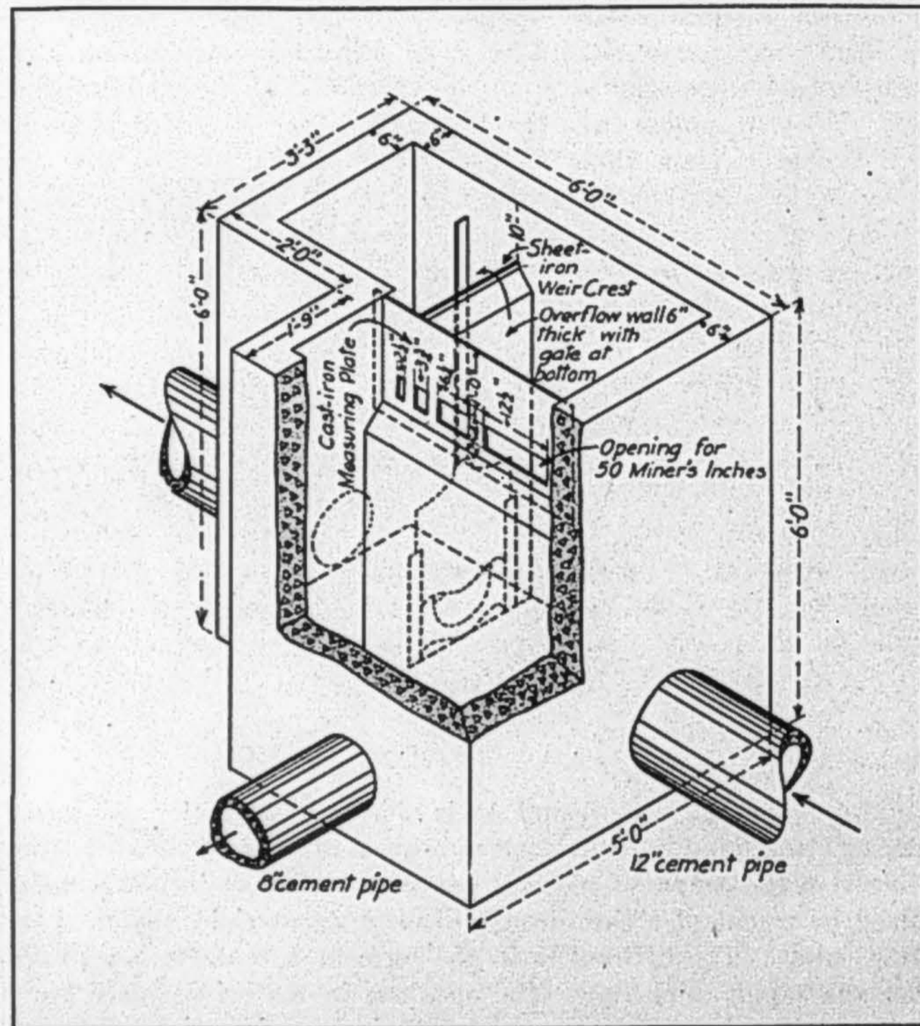
Fig. 3.—Drawing of Azusa hydrant
