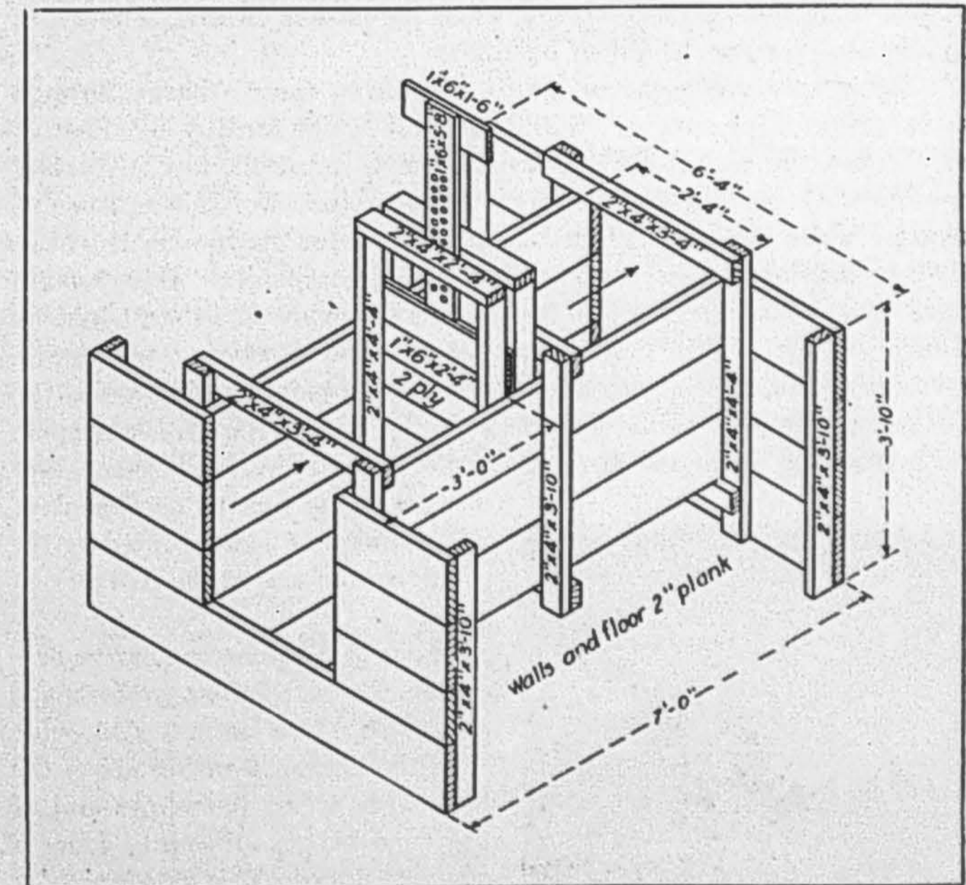
Fig. 17.—Drawing of submerged orifice headgate
