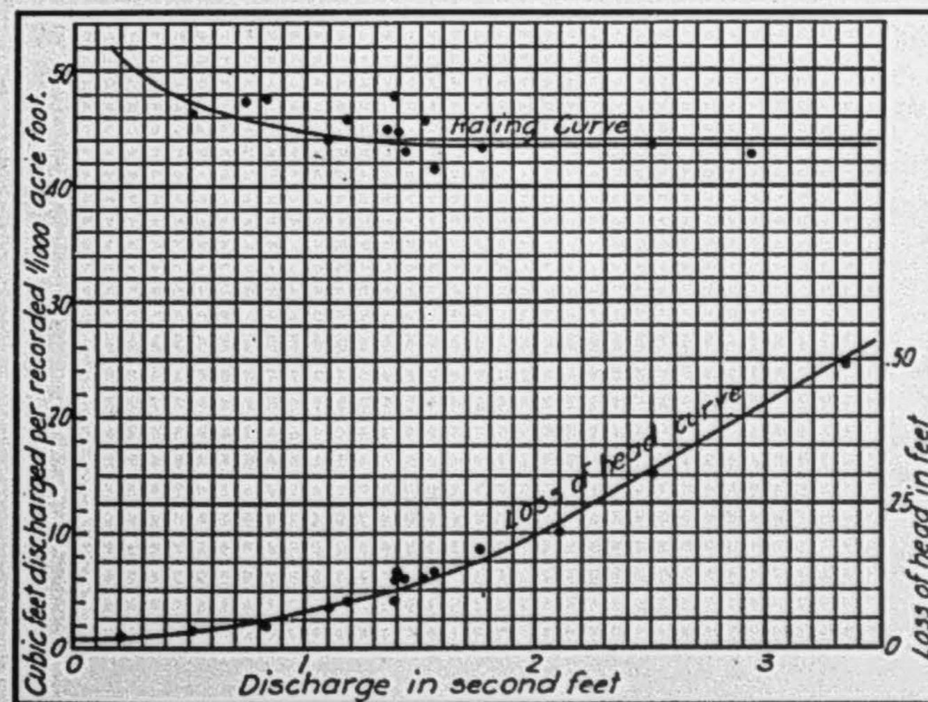
Rating Curve for Hill Meter
