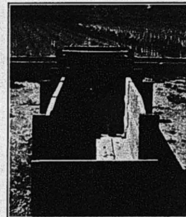
Fig. 22.—Photograph of installation of Grant-Michell meter
