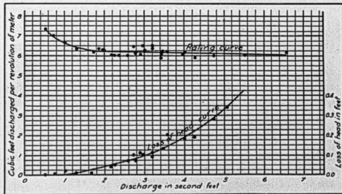
Rating Curve for Grant Michell Meter
