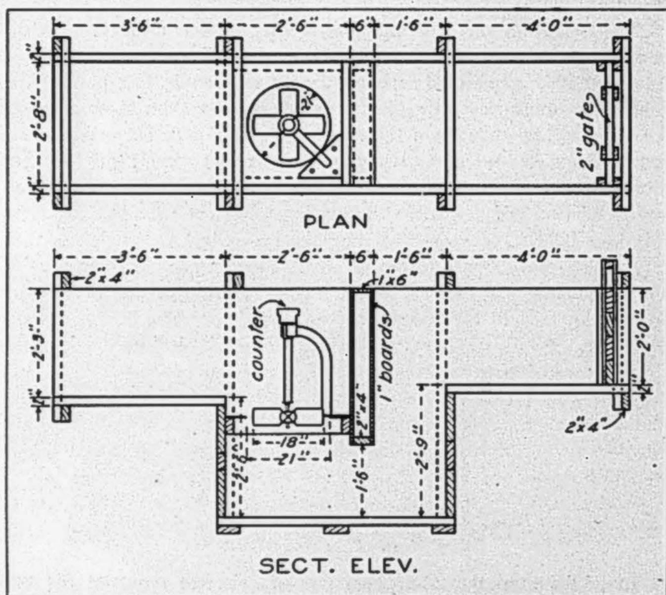
Fig. 21.—Plan and elevation of installation of Grant-Michell meter
