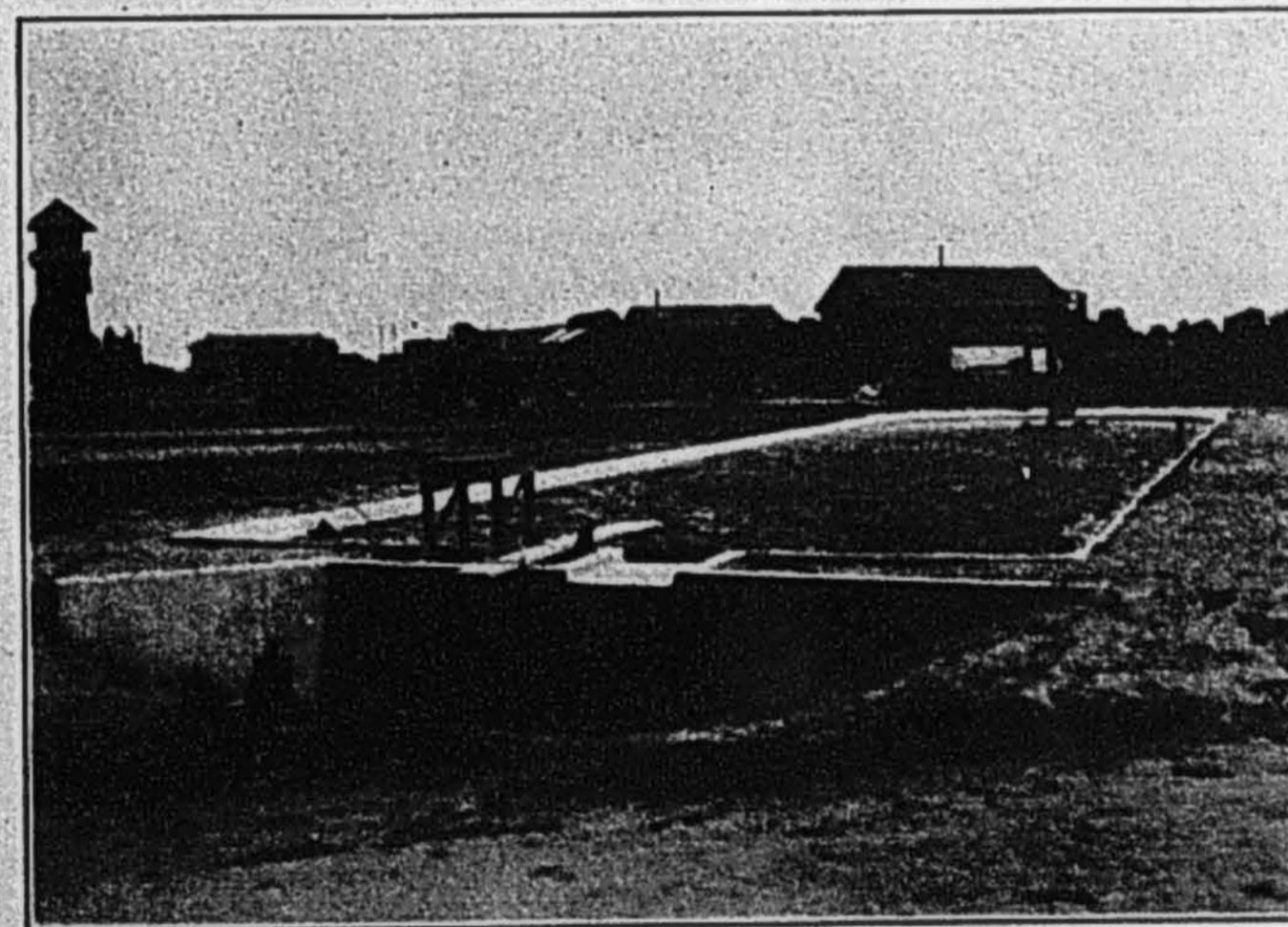
Fig. 1.—Reinforced concrete reservoir, Davis Field Laboratory
