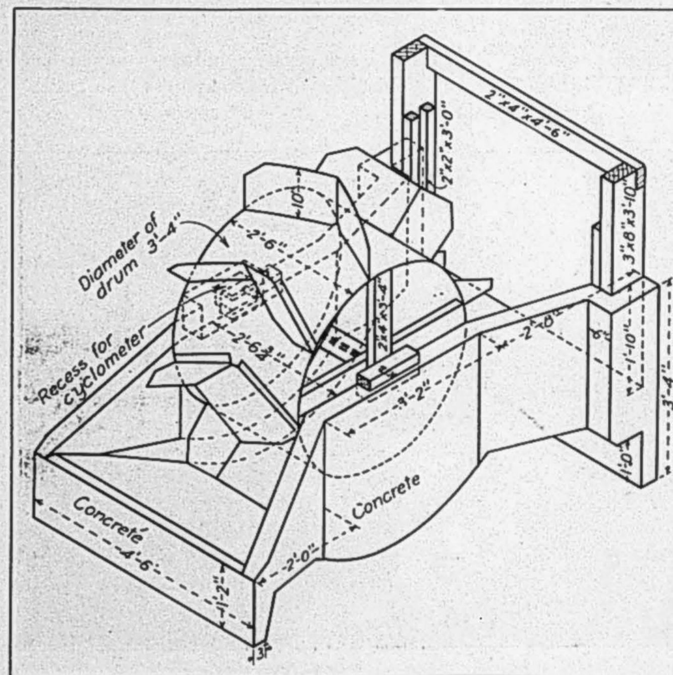
Fig. 19.—Drawing of Dethridge meter
