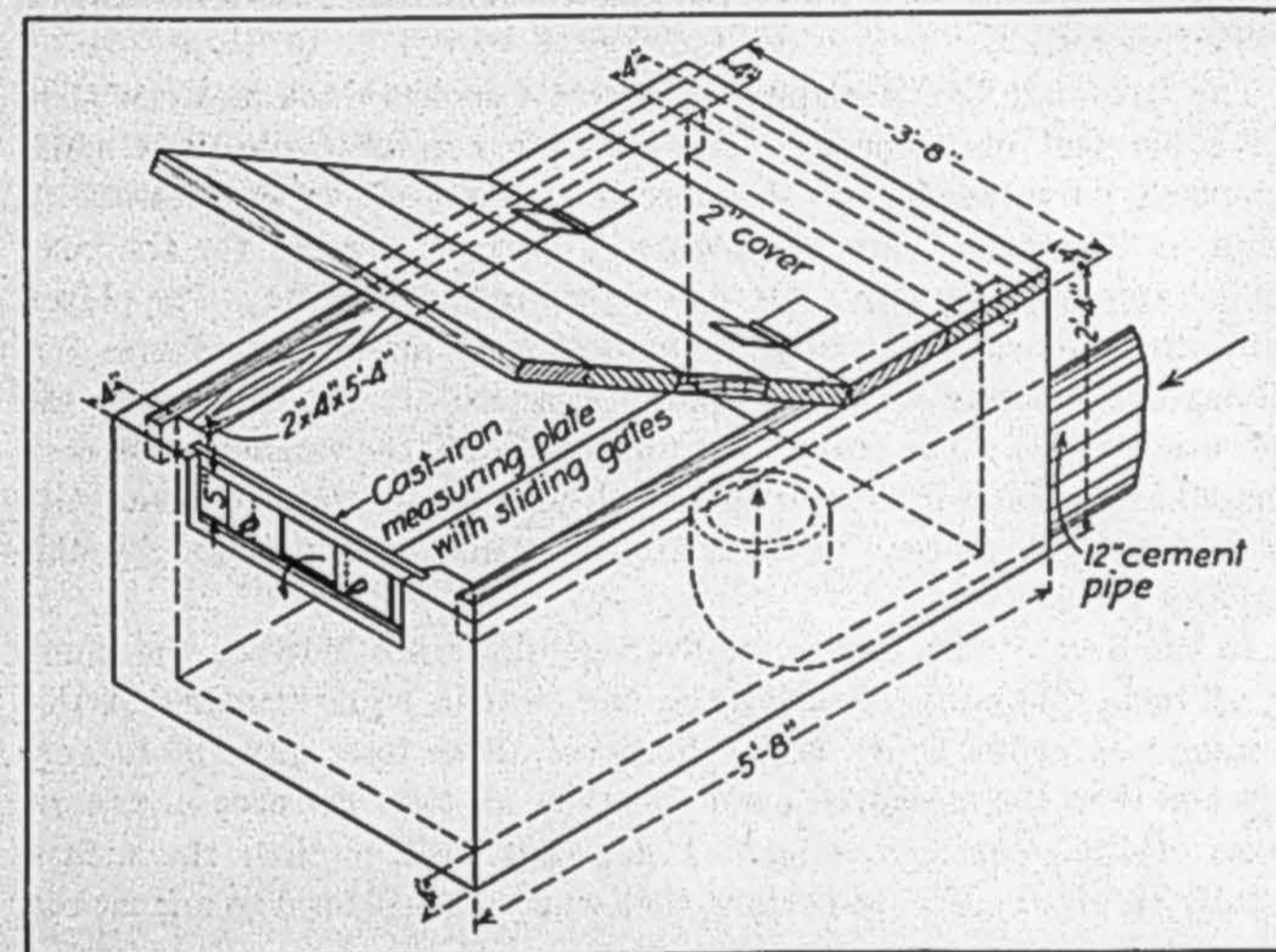
Fig. 7.—Drawing of Riverside measuring box
